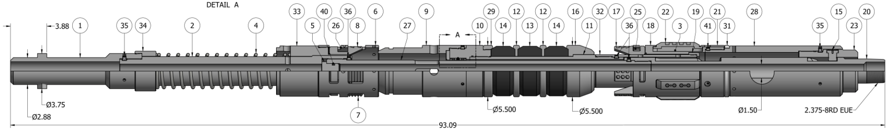
DETAIL A
