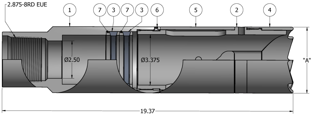
DIMENSIONAL DATA (INCHES)
